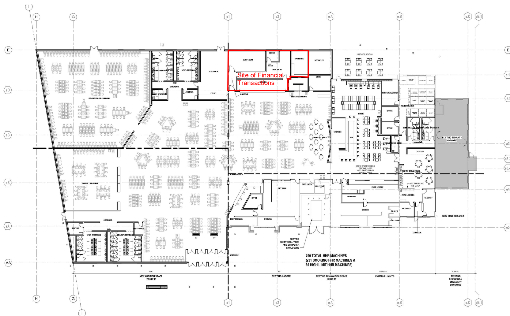
1 OVERALL FLOOR PLAN 3/32" = 1'-0"
