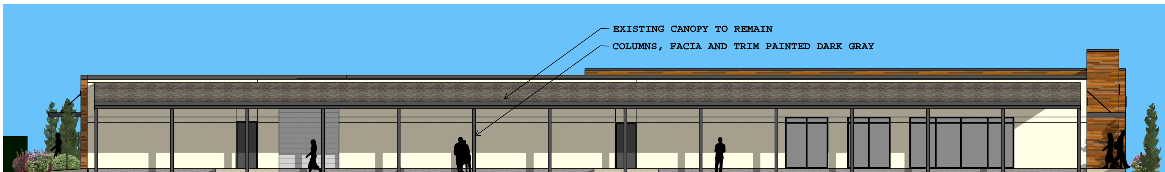
WEST ELEVATION
