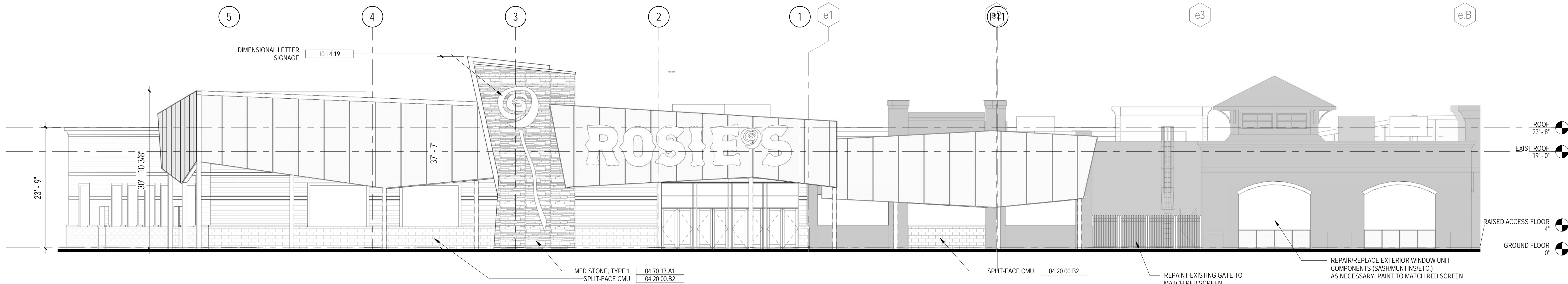
1 SOUTH ELEVATION 1" = 10'-0"
