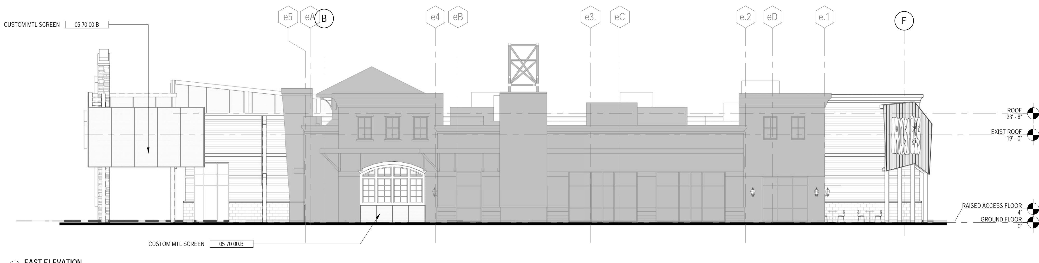
4 EAST ELEVATION 1" = 10'-0"
