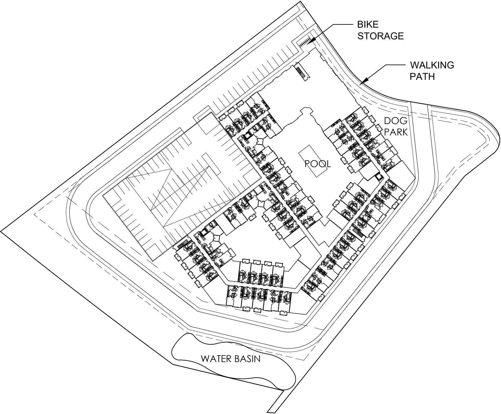
1 Site Plan - Ground Level Scale: 1" = 80'-0" Plan
