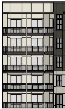
3 Courtyard 1 - North Elevation Scale: 1/32" = 1'-0"
