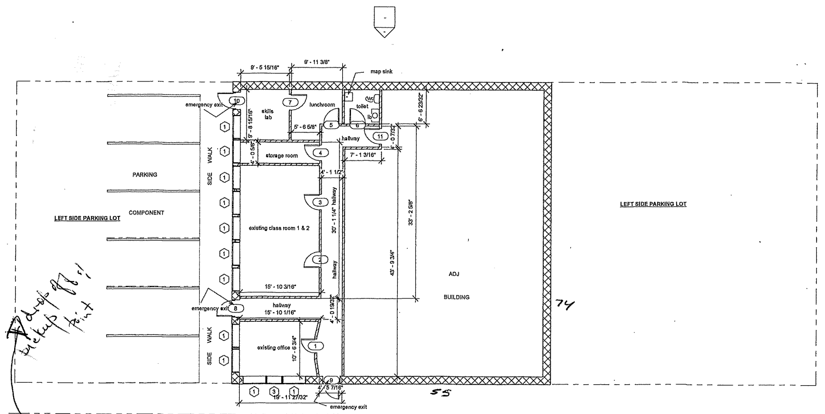
EXISTING FLOOR PLAN scale 1/4" = 1' - 0" 19 N MALLORY STREET
