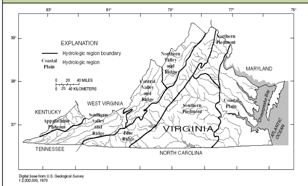
FIGURE 3.2: PHYSIOGRAPHIC REGIONS OF VIRGINIA
