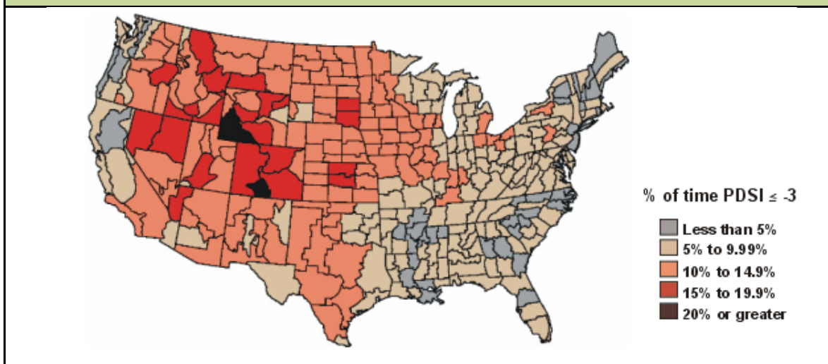
FIGURE 4.31: PALMER DROUGHT SEVERITY INDEX, 1895-1995 PERCENT OF TIME IN SEVERE AND EXTREME DROUGHT
