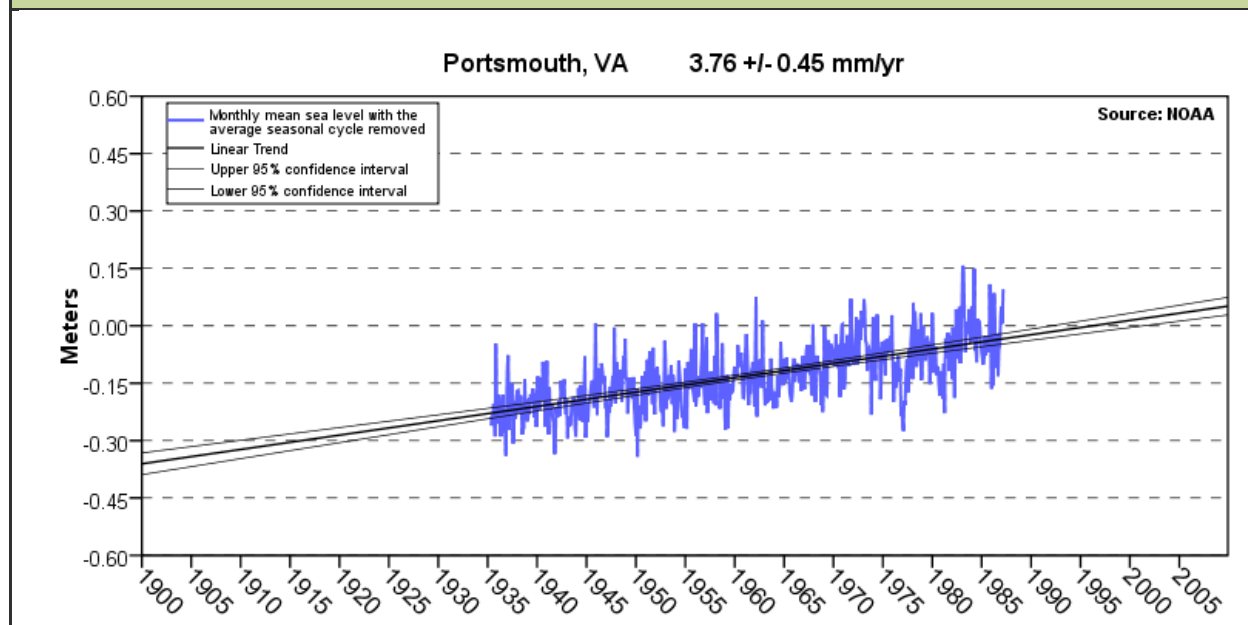
FIGURE 4.14: MEAN SEA LEVEL TREND, PORTSMOUTH, VIRGINIA
