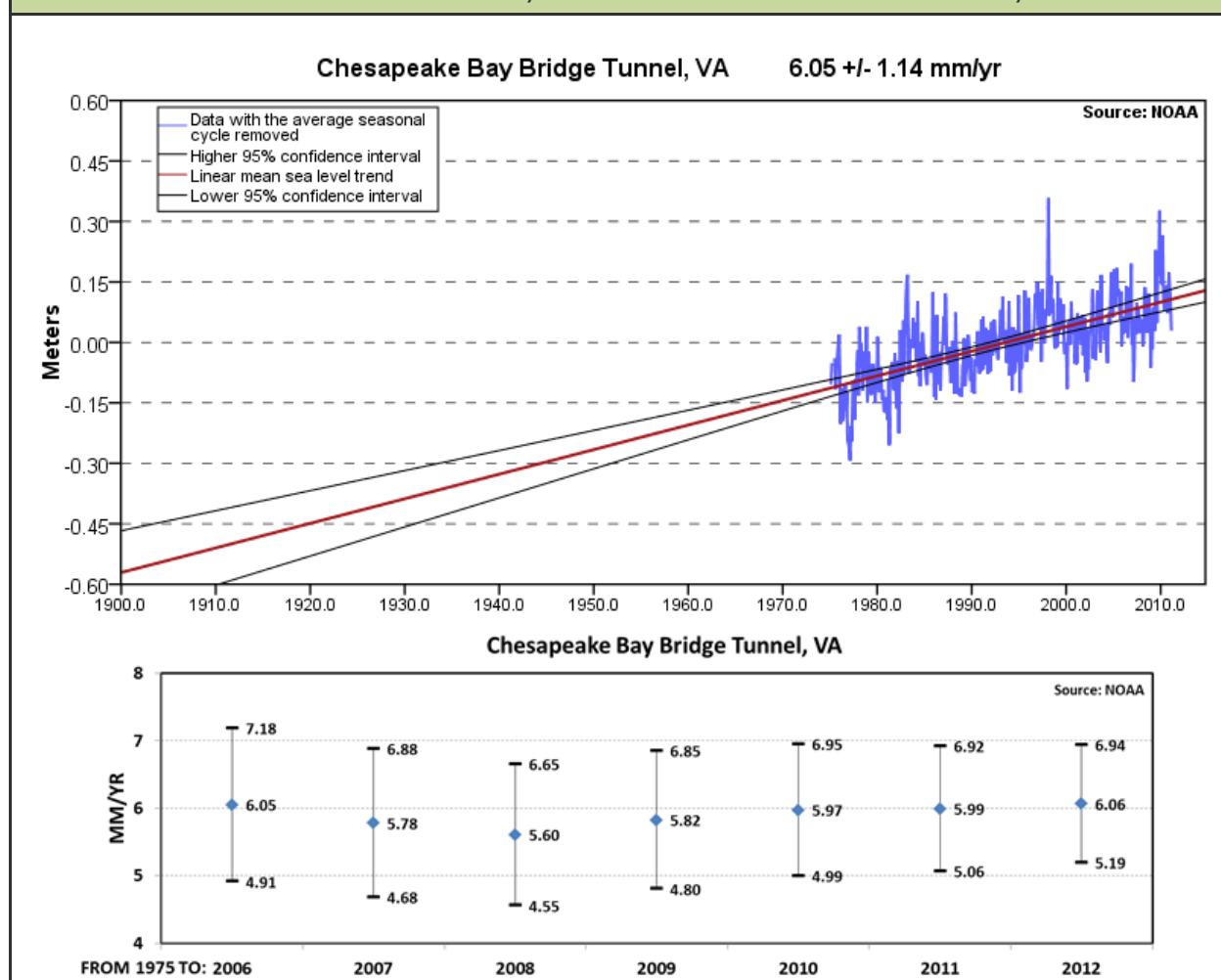
FIGURE 4.15: MEAN SEA LEVEL TREND, CHESAPEAKE BAY BRIDGE TUNNEL, VIRGINIA
