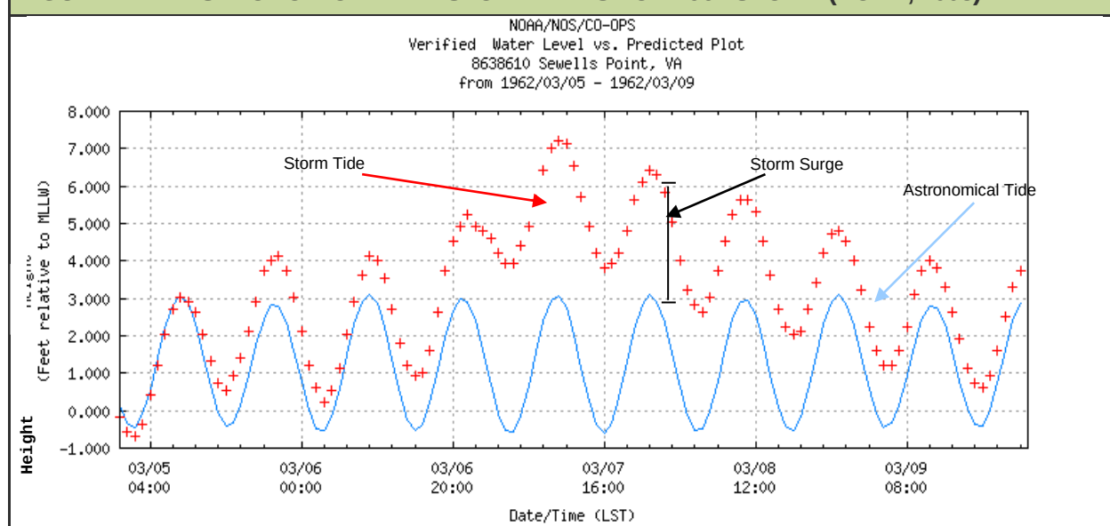
FIGURE 4.17: ASTRONOMICAL AND STORM TIDES FOR 1962 STORM (NOAA, 2008)
