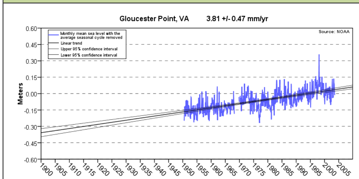
FIGURE 4.16: MEAN SEA LEVEL TREND, GLOUCESTER, VIRGINIA
