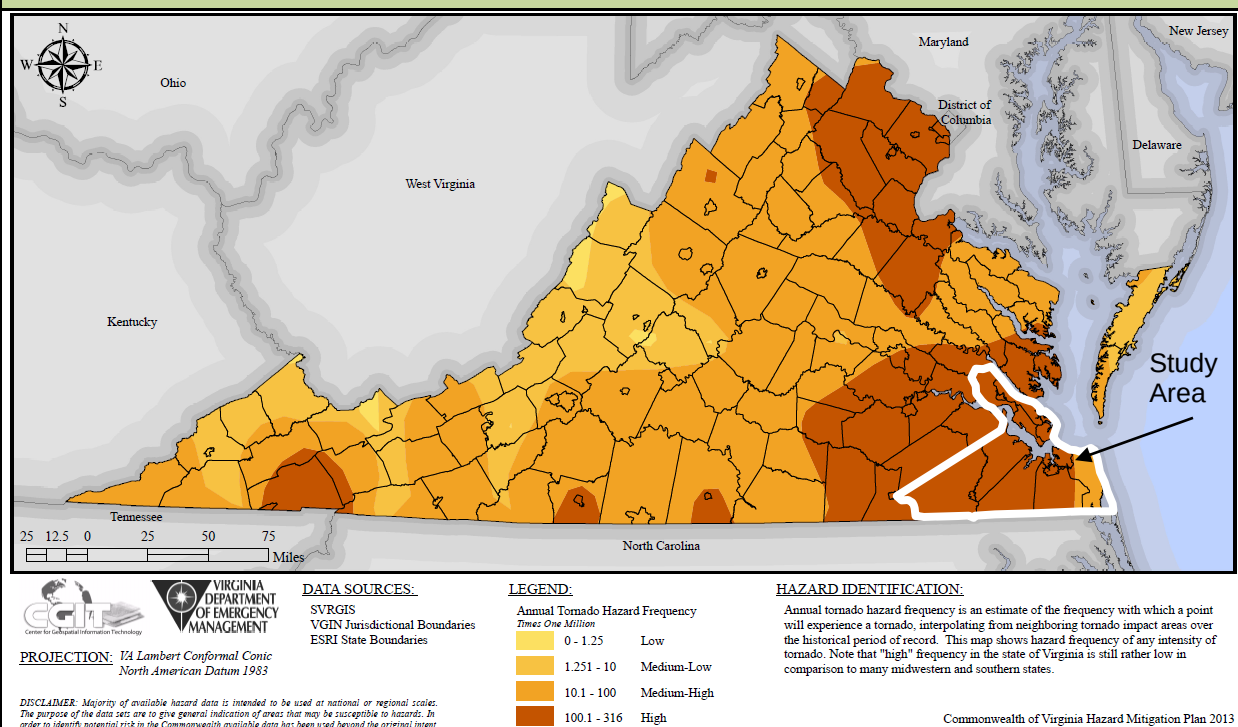
FIGURE 4.24: HISTORICAL TORNADO HAZARD FREQUENCY
