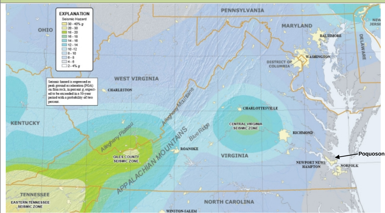
FIGURE 4.28: CENTRAL VIRGINIA SEISMIC ZONE
