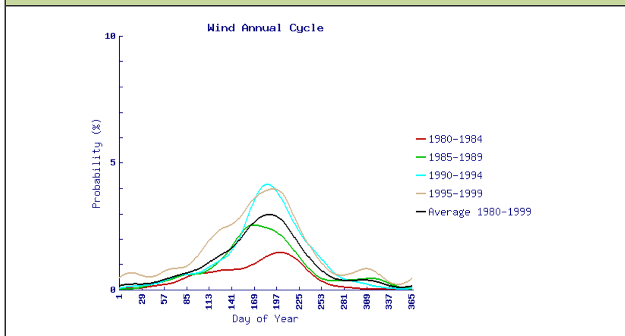
FIGURE 4.25: ANNUAL WIND CYCLE
